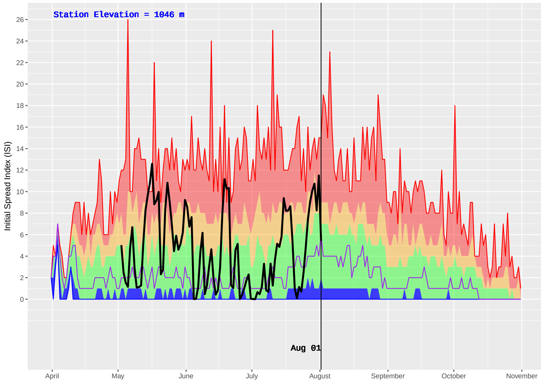
LIKELY RS (255) : Historical (1970–2016) and Current (2018) Daily Initial Spread Index (ISI)
