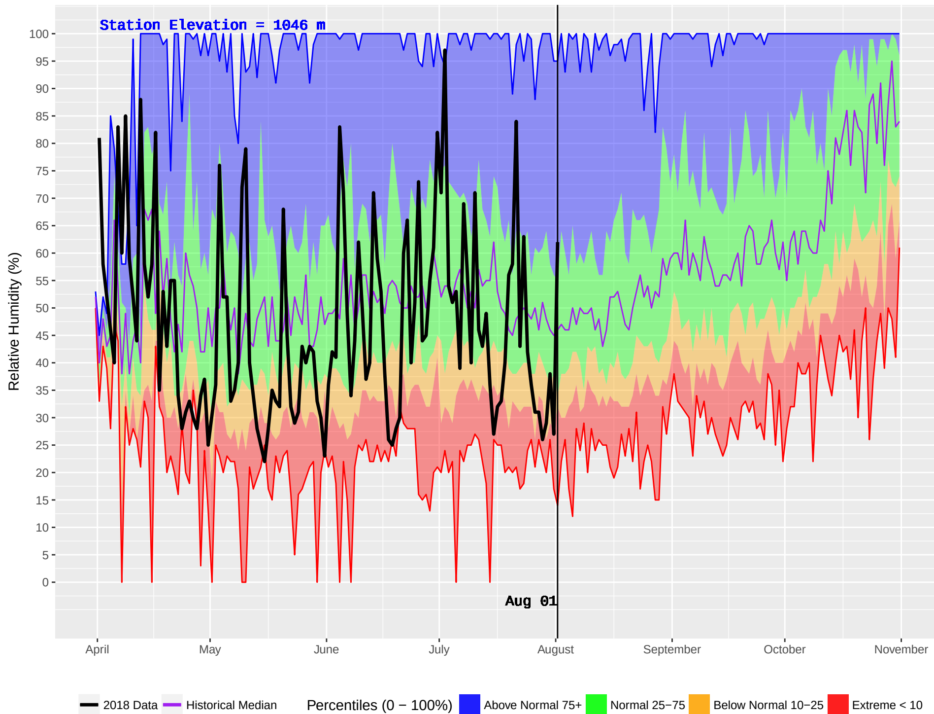
LIKELY RS (255) : Historical (1970–2016) and Current (2018) Daily Relative Humidity
