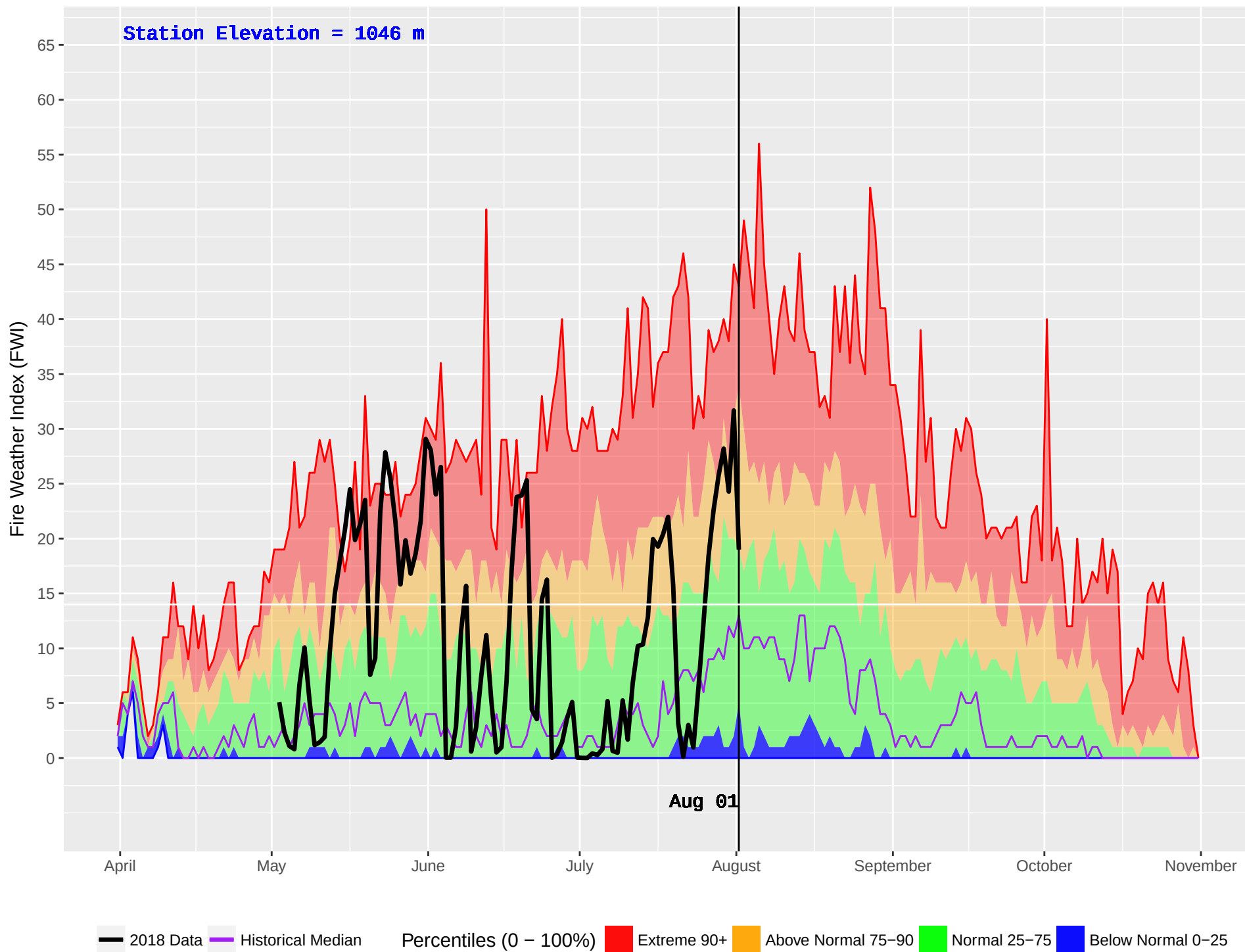
LIKELY RS (255) : Historical (1970–2016) and Current (2018) Daily Fire Weather Index (FWI)
