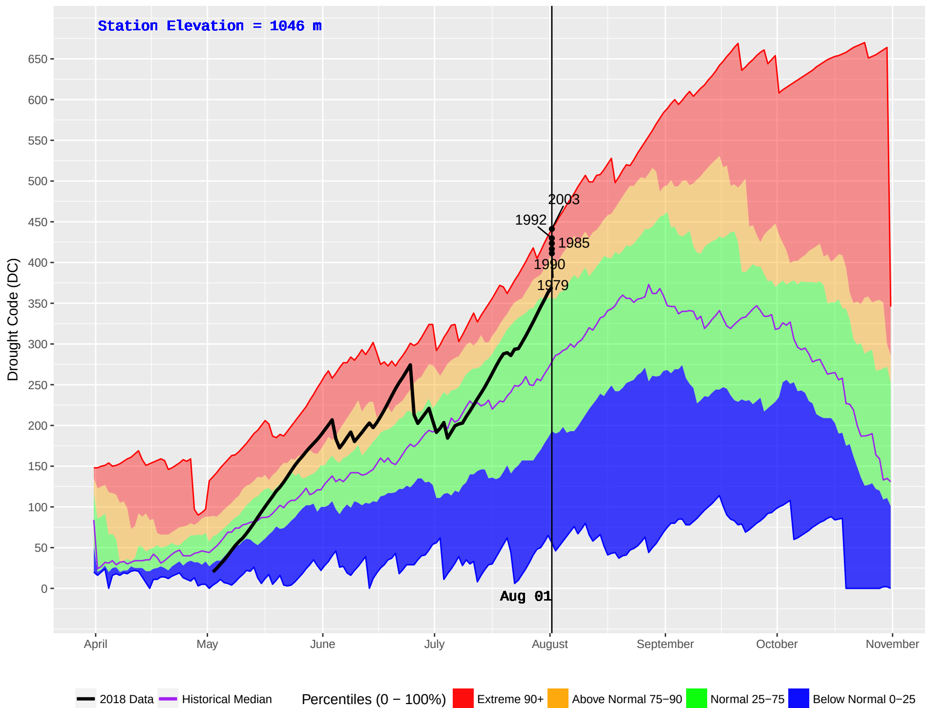
LIKELY RS (255) : Historical (1970–2016) and Current (2018) Daily Drought Code (DC)
